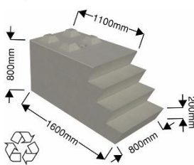
C3Cblock™ 1688TRL Trappstegblock Trappsteg
