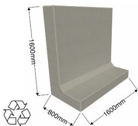
C3Cblock™ L-Block Specialblock
